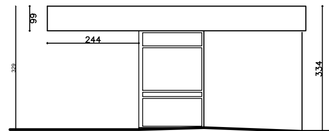
east elevation
